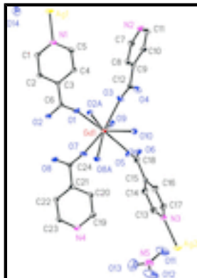
Fig. 1. The asymmetric unit of the title compound. Displacement ellipsoids are drawn at the 30% probability level. Additional symmetry related atoms are included to complete the coordination geometry around the Gd atom. [Symmetry code: (A) x, 1/2-y, 1/2+z .]
